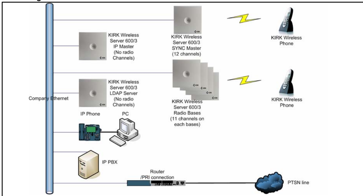
Figure 89 KWS600v3 Multi-cell installation with LDAP Server
